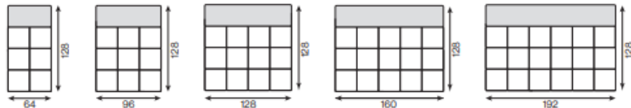
1-seater deep 1.5-seater deep 2-seater deep 2.5-seater deep 3-seater deep
